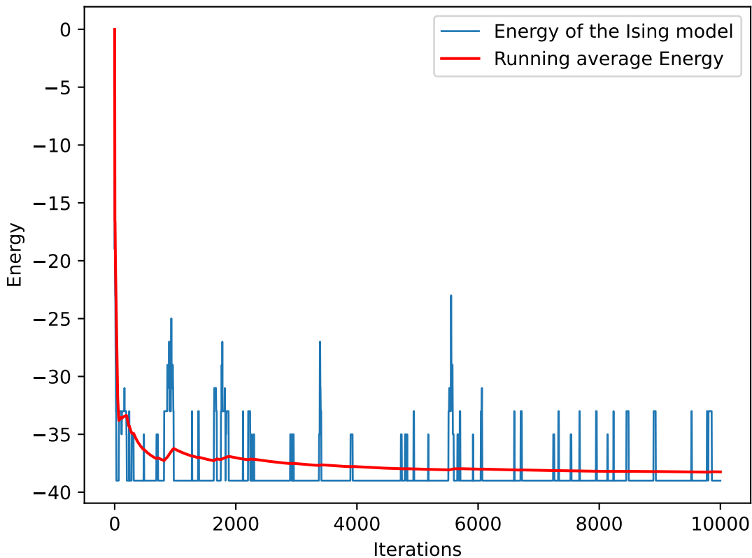
Evolution of a stochastic simulation of the 1D Ising model, at \beta = 1 J = 1 h = 1
